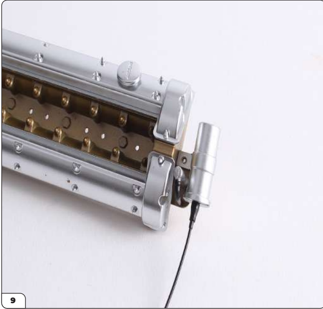
This shows the engine breather correctly fitted.
