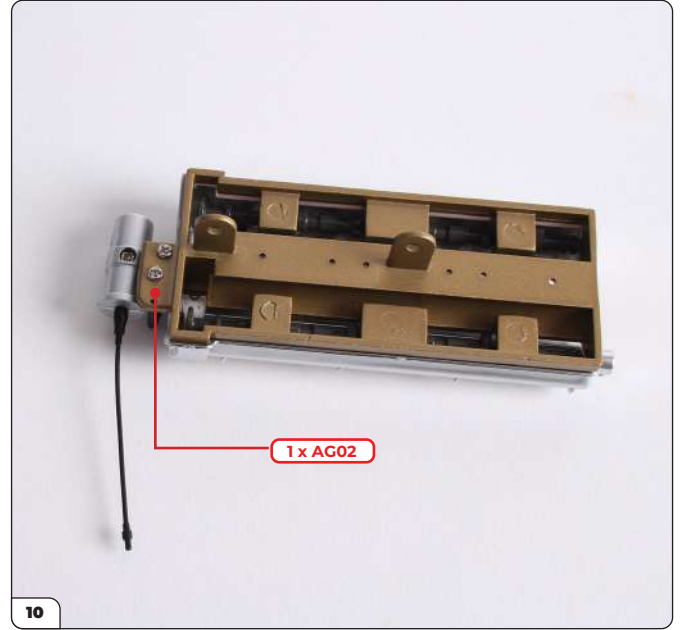
Secure in place from the reverse side using an AG02 screw.
