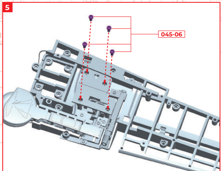
Fix the cover 045-01 with the 4 screws 045-06 that came with
