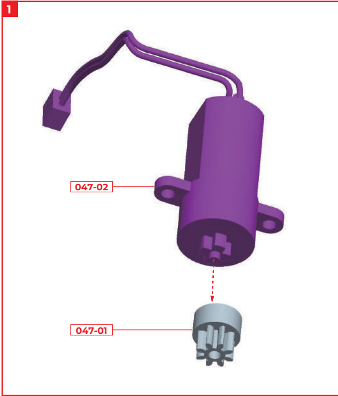
Fit gear 047-01 into motor 047-02. Pay attention to the direction
