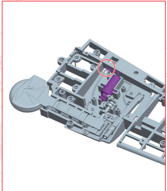
Fit the motor assembled in 1 into the right wing frame 044-01 assembled in stage 46. Pass the motor wire through the circled part.
